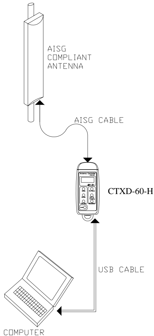
Figure 4. Controller Interconnection Showing Optional PC Interface
